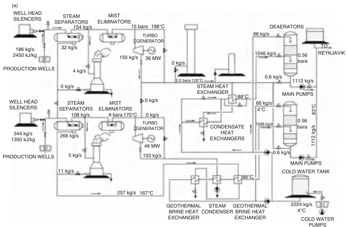
Figure 2.11 (a) Flow diagram of the Nesjavellir plant, Iceland. (b) Simplified flow diagram for the district heating in Reykjavik. Both diagrams are after Lund (2005) and reproduced by kind permission of Dr John W. Lund and the GeoHeat Center, Klamath Falls, Oregon.
