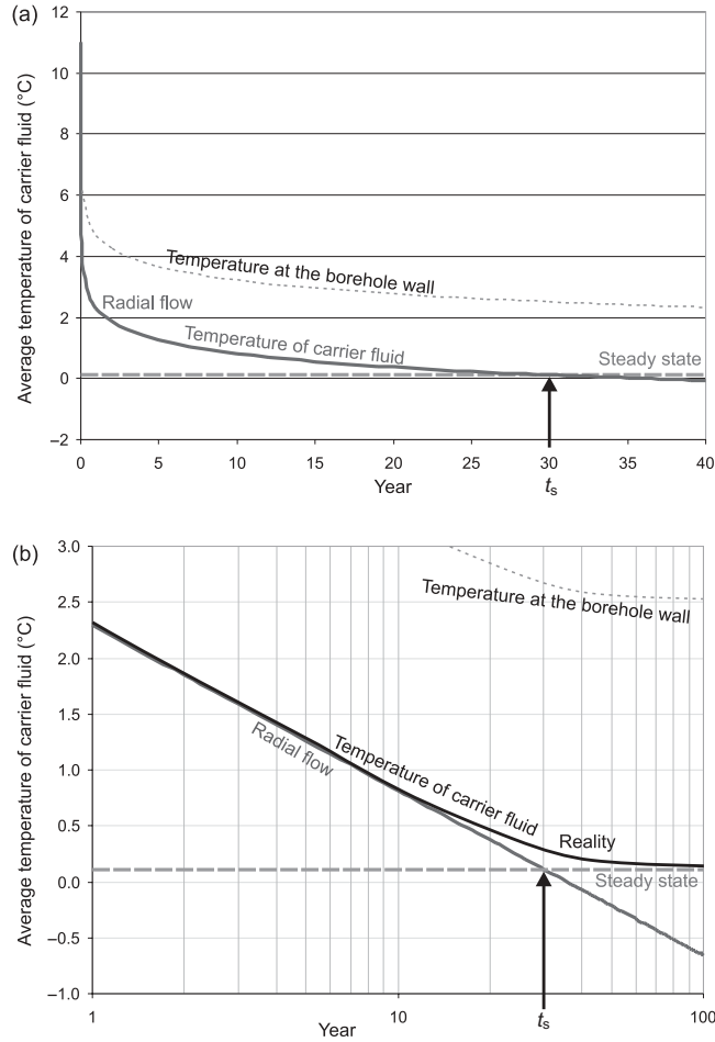
Figure 10.5 The development of average temperature (a) with time and (b) with \log_{10} (time) of the carrier fluid in a closed-loop borehole. Here, the borehole diameter is 126 mm, the constant heat extraction rate is 2 kW, R_b = 0.12 \text{ K m W}^{-1} , ground thermal conductivity 2.48 \text{ W m K}^{-1} , S_{VC} = 2.4 \text{ MJ m}^{-3} \text{ K}^{-1} and the undisturbed ground temperature 11^\circ\text{C} over the borehole's 100 m length. The diagram also shows the calculated temperature of the borehole wall ( 2.4^\circ\text{C} hotter than the carrier fluid).
