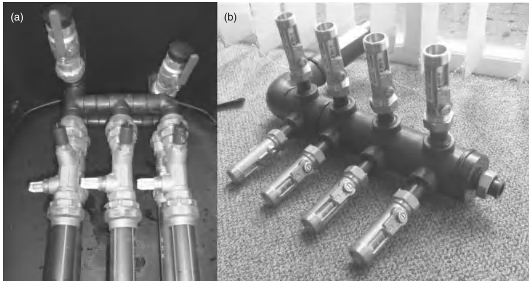
Figure 9.9 Photographs showing two types of carrier fluid manifold: (a) reproduced by kind permission of Water and Energy Field Services Ltd. ; (b) fitted with automatic flow balancing valves (photo by David Banks).
