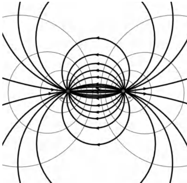
Figure 8.11 A well-doublet system, comprising an abstraction well (left) and a re-injection well (right); in this case there is no natural hydraulic gradient. Both the flow lines between the wells (thicker arrowed lines) and groundwater head contours (thinner lines) all form arcs of circles, making the scenario amenable to geometric analysis.
