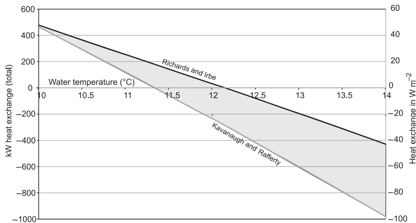
Figure 12.4 An example of a heat balance calculation for a 1-Ha lake ( 10000\text{m}^2 ), with an average extraterrestrial irradiance of 200\text{W m}^{-2} , a short-wave albedo of 8%, a moderately cloudy sky, an air temperature and relative humidity of 14^\circ\text{C} and 60% and a wind speed of 4\text{m s}^{-1} . The graph shows the approximate effect of lake water temperature on heat fluxes. The two lines indicate that the evaporative component of the heat budget is calculated by the algorithms cited by Richards and Irbe (1969) and Kavanaugh and Rafferty (1997), respectively.
