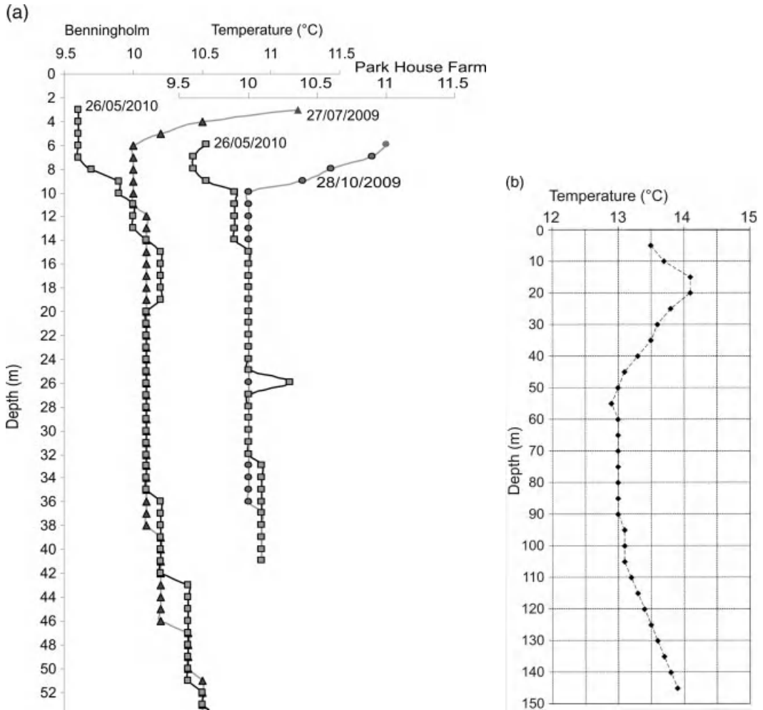
Figure 3.9 (a) 'Normal' temperature profiles from two water wells (Benningholm and Park House Farm) in the Chalk aquifer of East Yorkshire, UK, based on data from Russell (2010). Note that the top 10m of each profile appear to be affected by seasonal temperature fluctuations (the July and October profiles show a summer 'pulse' of heat entering the top of the column, the May profiles show a residual cold 'pulse' from winter). Below 10m, the temperature is stable and increases slowly due to the geothermal gradient. (b) A temperature profile from a closed-loop borehole in London, illustrating the effect of the urban environment in enhancing near-surface temperatures and reversing the natural geothermal gradient down to a depth of c. 50m. Reproduced by kind permission of Econic Ltd. and Neo-Energy (Sweden) Ltd.
