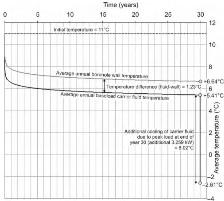
Figure 10.15 The evolution of average carrier fluid temperature over 30 years for a 100-m-deep, closed-loop ground source heat borehole, delivering a peak heat load of 6 kW with a \text{COP}_H of 3.5. The solid curve shows the annual average trend of carrier fluid temperature (corresponding to a continuous heat extraction of 1.027 kW), while the final downward ‘spike’ shows the approximate minimum fluid temperature under short-term (24 h) peak heating load, superimposed on the base-load trend after 30 years.
