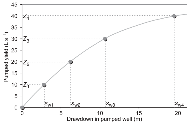
Figure 8.4 Plot of yield versus drawdown for step testing. For any yield Z , we can predict a corresponding drawdown ( s_w ) after 2 h of pumping.
